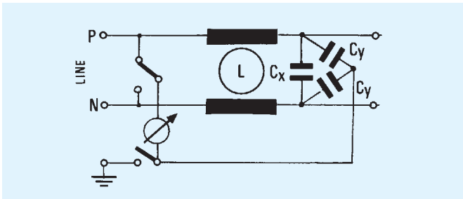
Fig.13 Data and measurement method relevant to leakage current of the equipment (including filter) are based on EN 60335-1. The formula for the approximate calculation of the maximum leakage current of a single-phase filter with a delta capacitive construction (Fig.13) is as follows:
