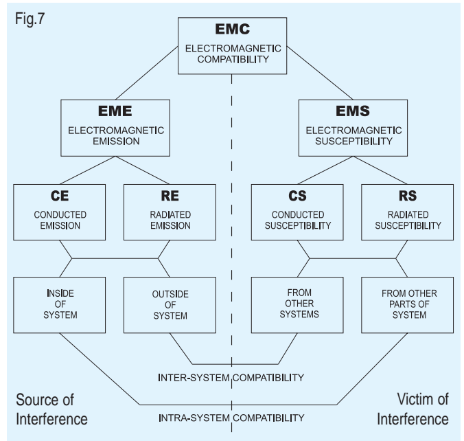
Fig.7 shows the EMC concept.
