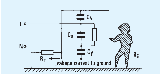
Fig.12 Besides the leakage current due to the filter, that associated with the equipment must be taken into account. All these currents are cumulative at the protective earth conductor. This total current cannot exceed the limit value, set by the safety specifications of the various national regulatory bodies and this depends on the type of equipment under consideration.
