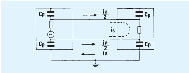
Fig.2 i_s = differential mode interference current (symmetrical) i_a = common mode interference current (asymmetrical) C_p = stray capacitance
