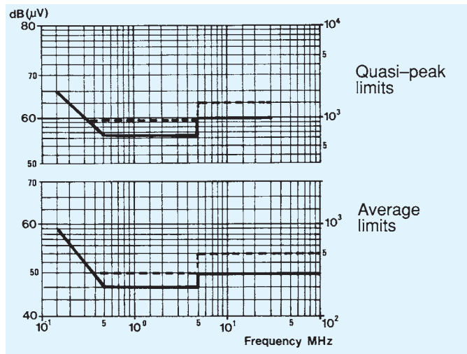
Fig.4 ——— Hand driven electric tools - - - - Household appliances
